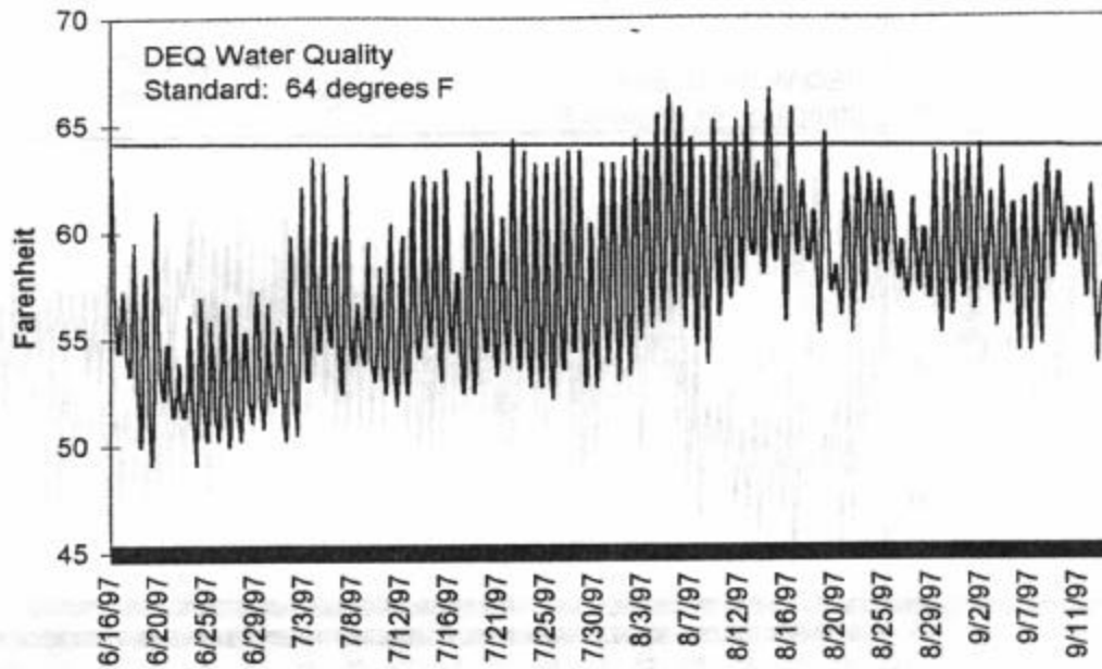
Water Temperature for West Creek: Summer 1997
