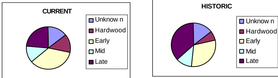
Figure 3-2: Seral Stage Distribution
